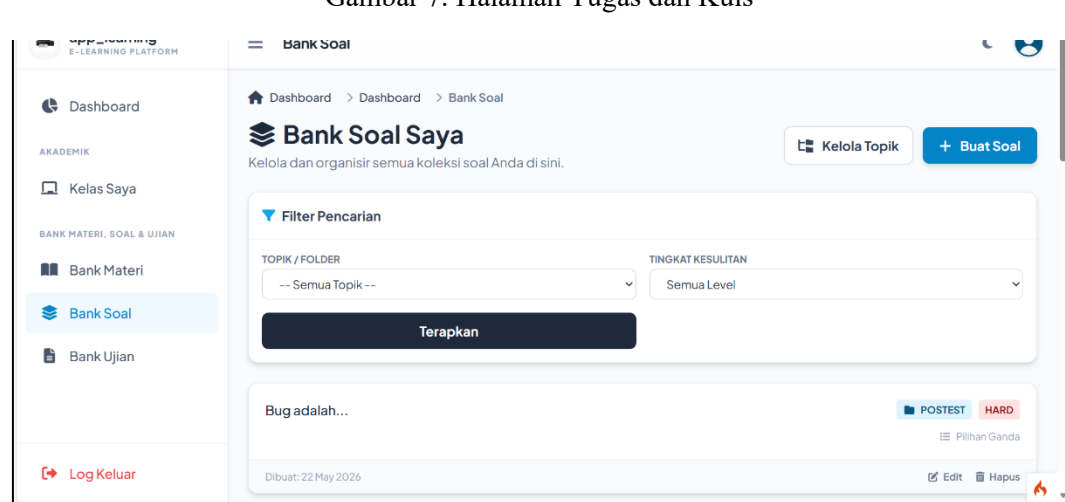
Gambar 8. Halaman Soal
