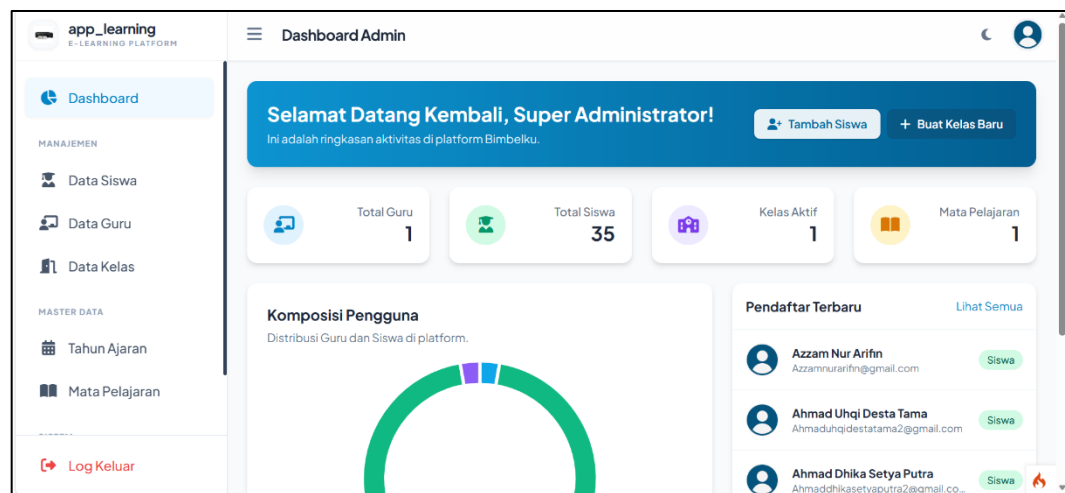
Gambar 9. Halaman Admin
