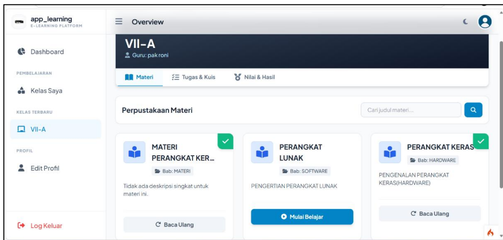
Gambar 6. Halaman Materi
