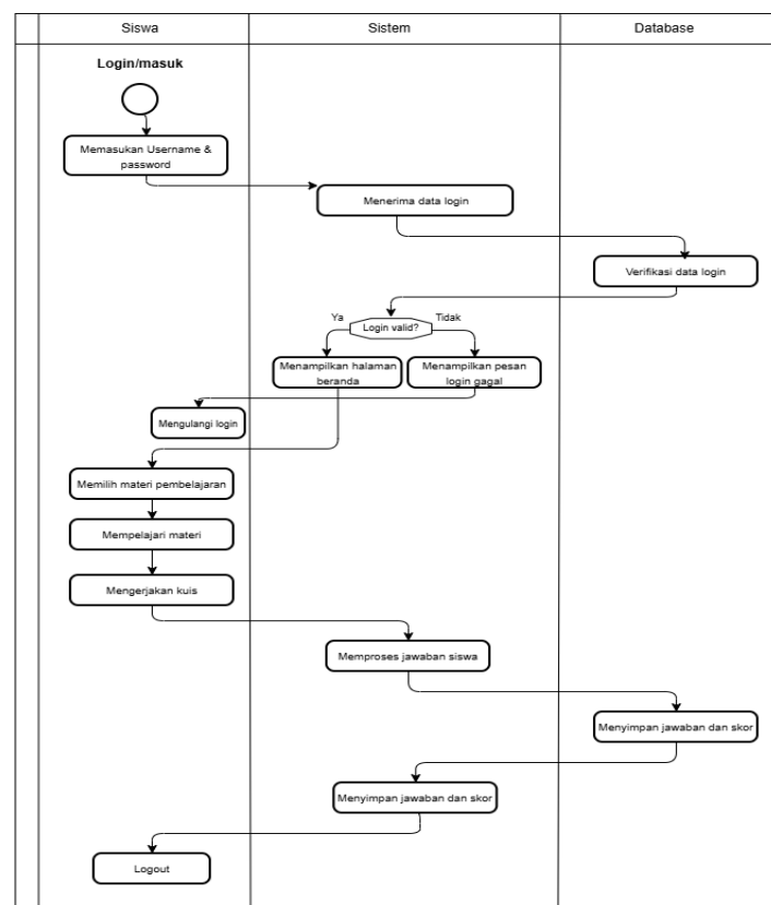
Gambar 2. Activity Diagram
